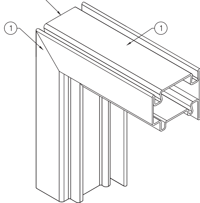
FRAME CORNER CONNECTION
