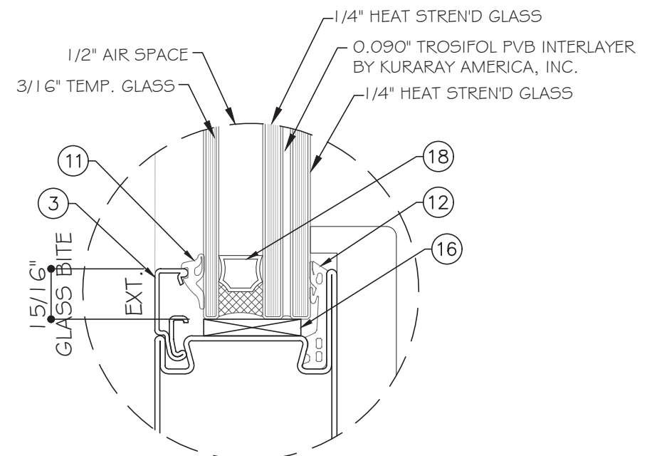
GLASS TYPE 'A' 1 - 1/2" NOMINAL OVERALL
